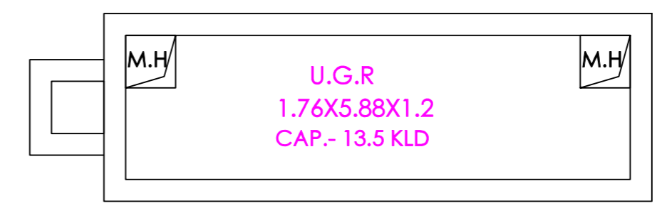
UGR DETAIL SCALE- 1:50
